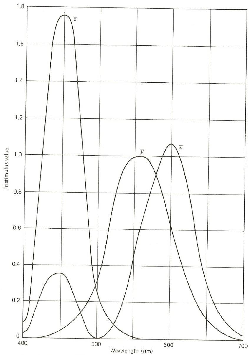
Figure 3.6 1931 CIE color matching functions for the XYZ system.
