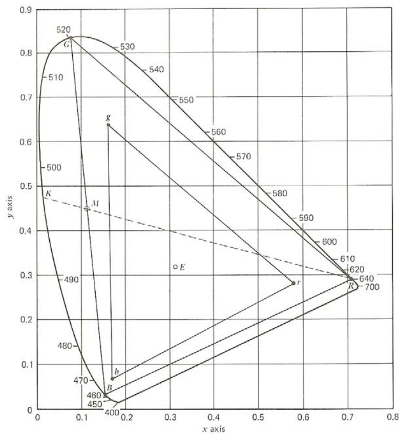
Figure 3.9 Chromaticity diagram showing the area covered by three monochromatic
