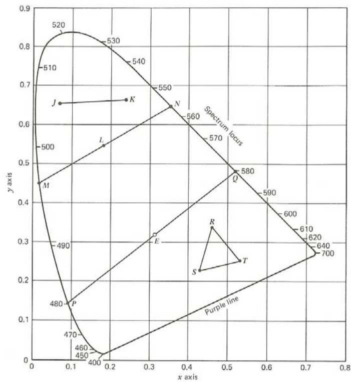
Figure 3.8 CIE chromaticity diagram illustrating various features of color mixing.
